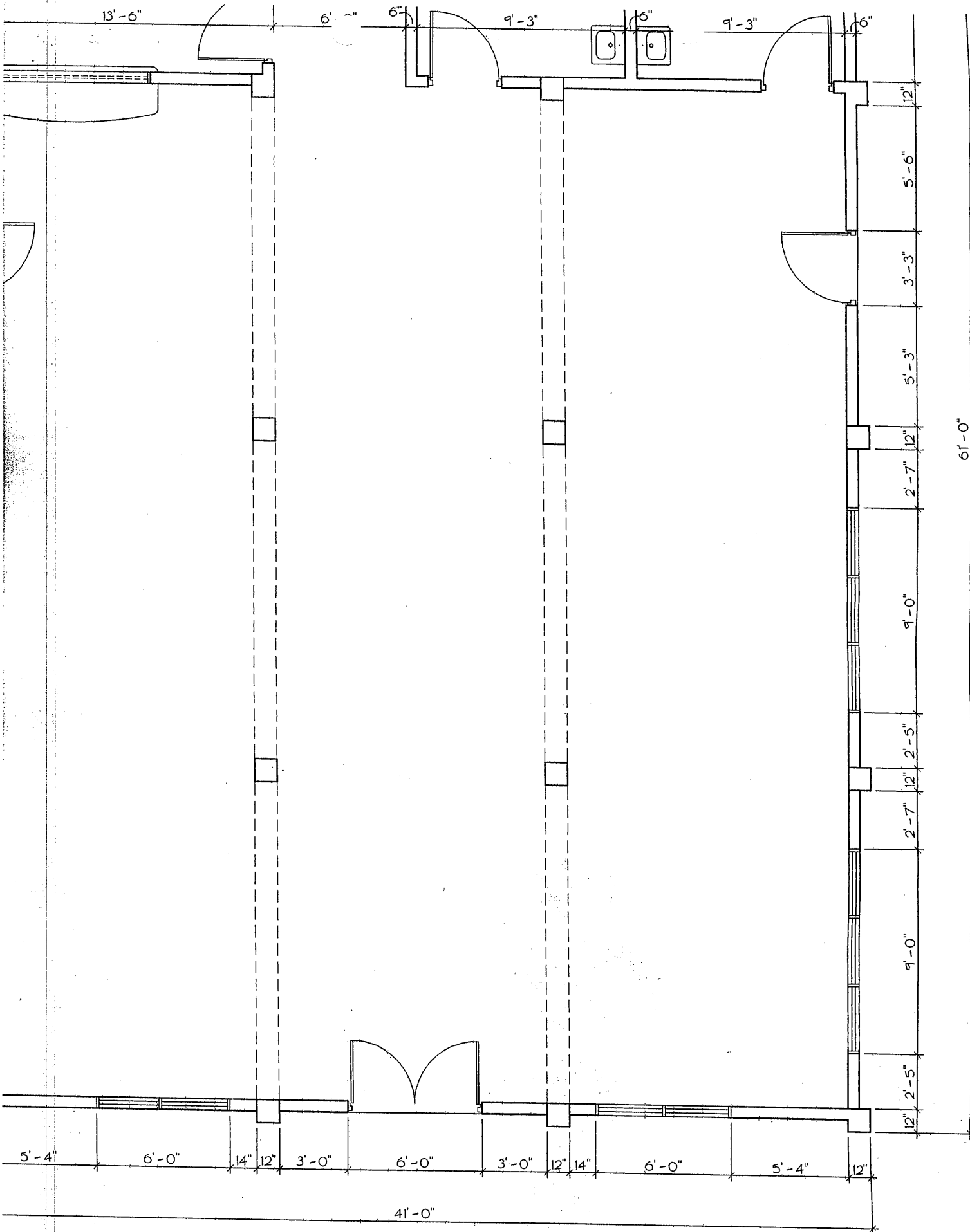
COMMUNITY CENTER - FLOOR PLAN SCALE: 1/4" = 1'-0"
